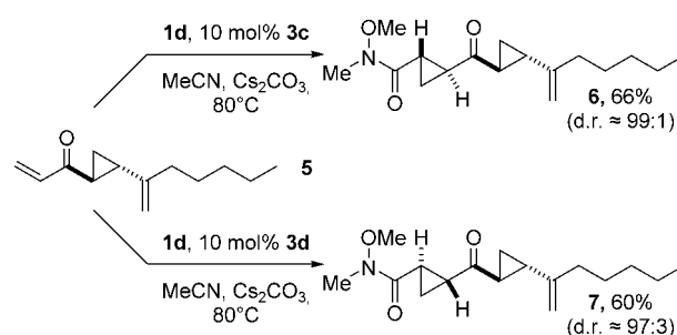
Scheme 2. Synthesis of biscyclopropanes.
