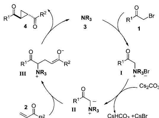
Scheme 1. Proposed catalytic cycle.
